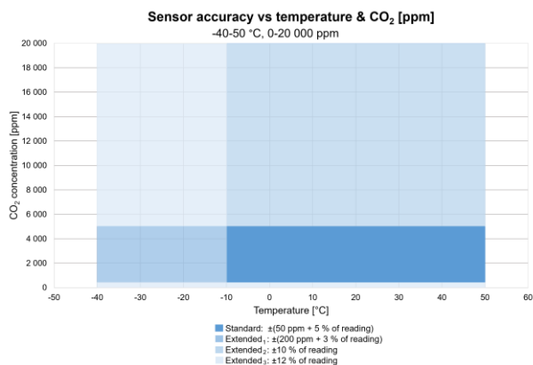
Figure 3. Accuracy over temperature and CO 2
