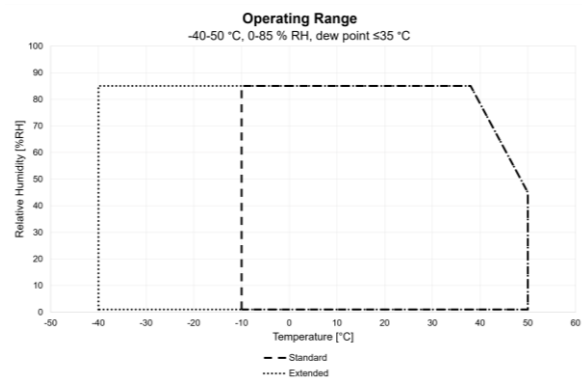
Figure 4. Operating range
