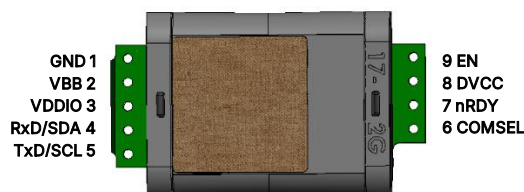
Figure 1. Pin configuration of Senseair Sunlight CO 2 2%
