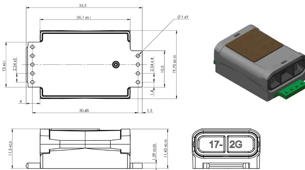
Figure 2. Dimensions of Senseair Sunlight CO 2 2%
