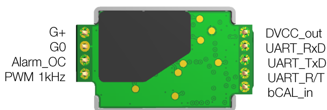
Figure 2. Pin assignment
