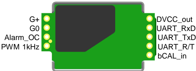
Figure 2. Pin assignment
