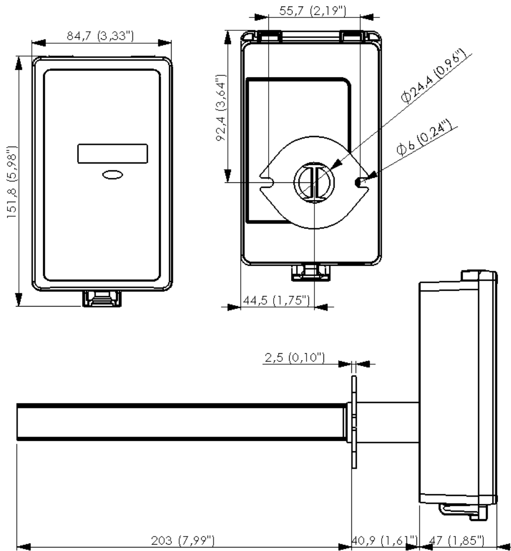
Figure 7 The dimensions of the sensor in mm and (inches)
