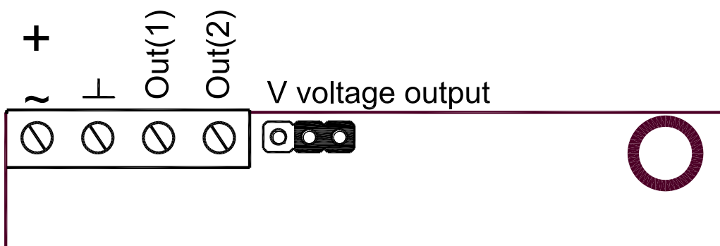
Figure 6 Enlarged picture of the PCB with the jumper set to voltage output (right position)
