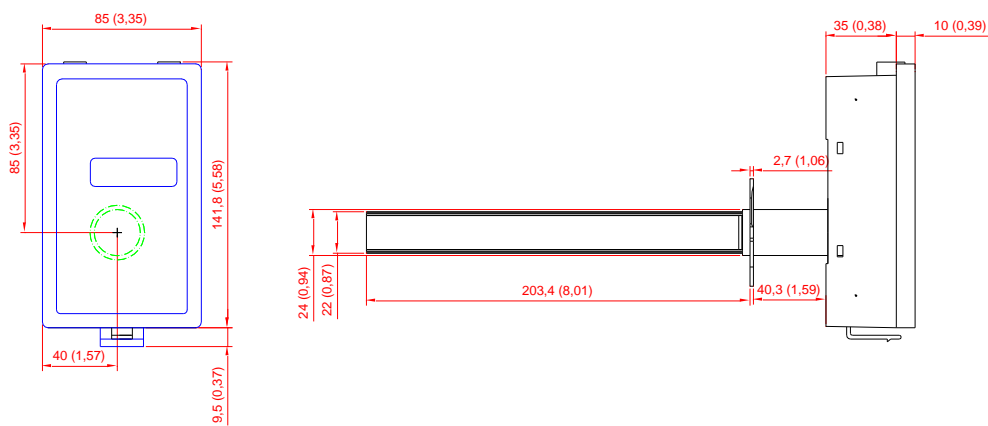
Dimensions of sensor in mm and inches
