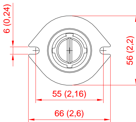
Dimensions of sampling probe in mm and inches
