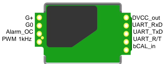
Figure 2. Pin assignment
